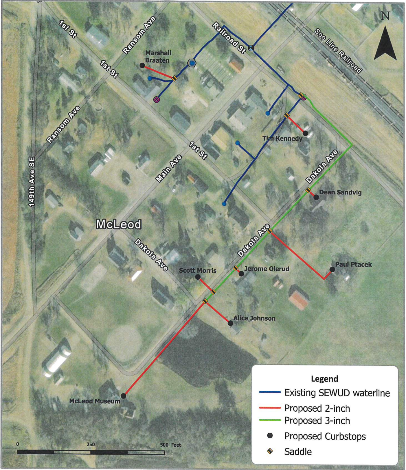
Figure 1 CITY OF MCLEOD NW 1/4 OF T134N R53W S25 SOUTHEAST WATER USERS DISTRICT
